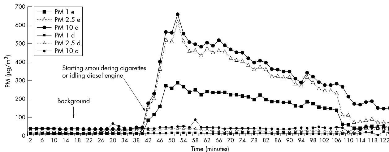
Figure 1 Particulate matter (PM) production from environmental tobacco smoke (e) and an ecodiesel engine (d) (three smouldering cigarettes or an idling engine for 30 minutes in a 60 m 3 garage).
