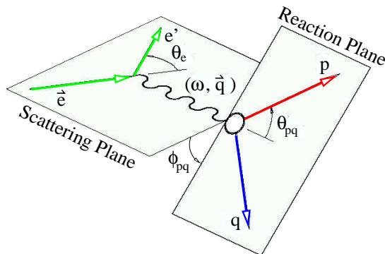
Figure 2: Kinematics of the D(\vec{e}, e'p)n reaction.
