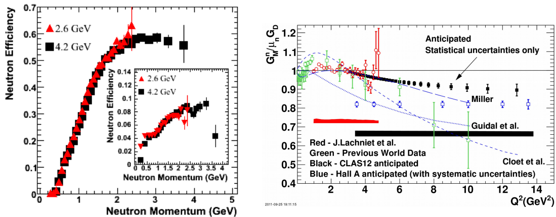
Figure: The left panel shows the results of the neutron detection efficiency for the CLAS6 electromagnetic calorimeters and the TOF system (inset). The right panel shows the magnetic form factor of the neutron normalized to the dipole form factor with results from other measurements and theoretical curves.
