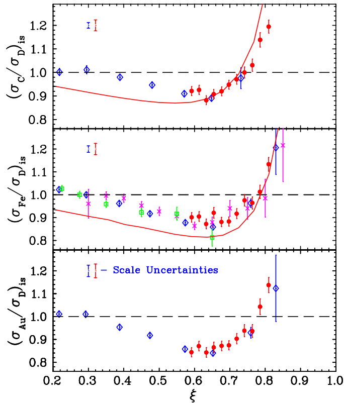
Figure 14: Comparison of nuclear to deuterium cross sections for data collected in the resonance region and the DIS region. The solid circles are Jefferson lab data taken in the resonance region and the open markers are the data taken in the DIS region at SLAC and BCDMS. As it can be seen the resonance data are in agreement with DIS data.
