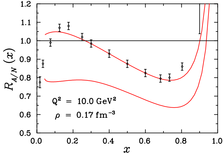
Figure 4: Ratios of the spin-independent and spin-dependent nuclear to nucleon structure functions at nuclear matter density [2]. The top curve is the ratio F_{2N}^A/F_{2N} for nuclear matter. Model predictions for the polarized EMC effect, g_{1p}^A/g_{1p} , is shown by the lower curve.
