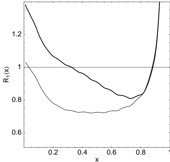
Figure 5: The ratio Eq. (2) at scale Q^2 = 10 \text{ GeV}^2 for nuclear matter in the model of Smith and Miller [4]. The heavy line is the full calculation for nuclear matter, which includes sea quarks. The light line is the effect calculated using only valence quarks at the model scale.
