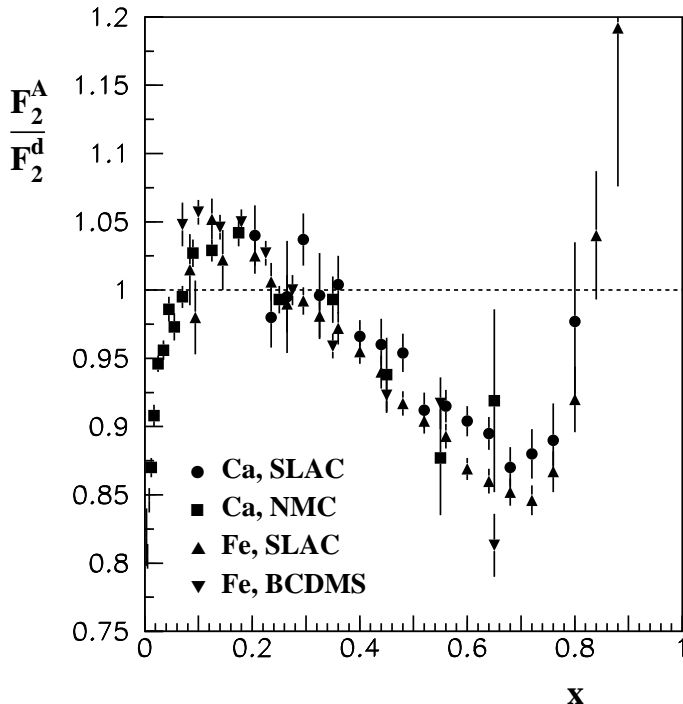
Figure 1: Experimental data for the EMC effect in the unpolarized structure function F_2 for ^{40}\text{Ca} and ^{56}\text{Fe} taken at NMC, SLAC and BCDMS.
