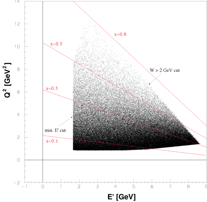
Figure 6: The plot shows the kinematic coverage of the intended measurement.
