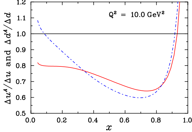
Figure 3: Ratio of the quark distributions in {}^7\text{Li} to the corresponding free distributions, at a scale of Q^2 = 10 \text{ GeV}^2 . The solid line represents \Delta u^A(x)/\Delta u(x) and the dot-dashed line \Delta d^A(x)/\Delta d(x) [2].
