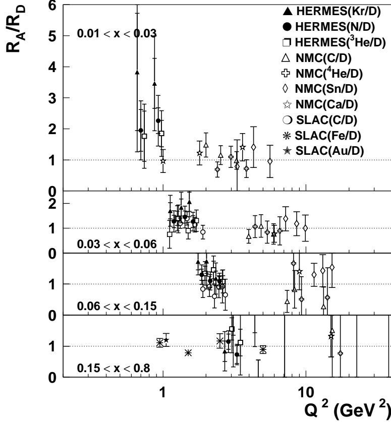
Figure 9: The ratio R_A/R_D for several nuclear targets with respect to deuterium as a function of Q^2 [23].
