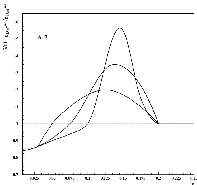
Figure 2: The figure shows the calculations of nuclear shadowing and modeling of the enhancement for the non-singlet combinations of spin structure functions. Three curves show three scenarios of the enhancement for {}^7\text{Li} , which depends on the cross-over point between the regions of shadowing and enhancement.
