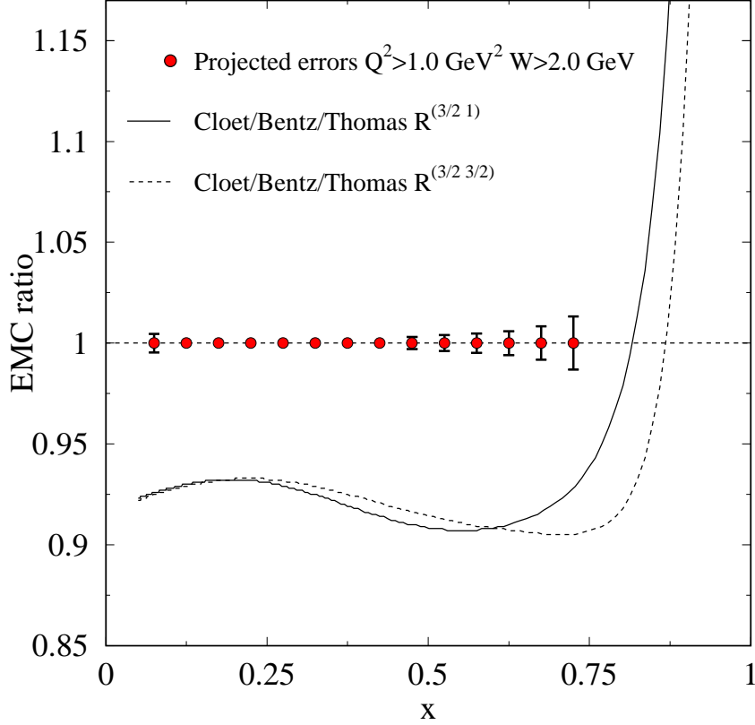
Figure 13: Projected statistical uncertainties for the ratio g_1^{p^{7Li}}/g_1^p as a function of x ; see text for details. Also shown is (solid line and dashed line) the predictions by [3] specifically for {}^7Li .
