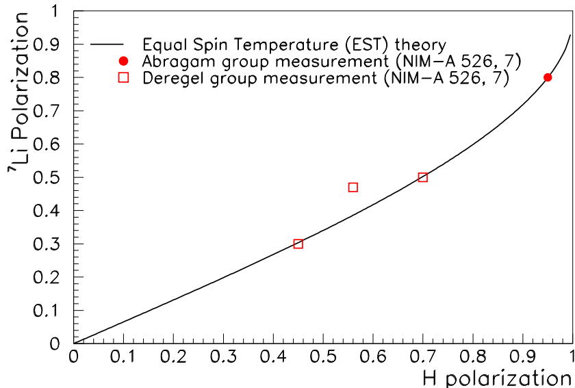
Figure 8: The polarization of {}^7\text{LiH} versus that of proton. The curve is the theoretical prediction from the EST theory.
