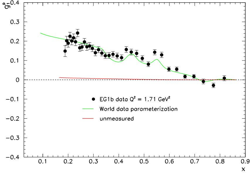
Figure 7: The figure compares the unmeasured contribution to g_1^p along with the EG1b results for g_1^p for Q^2 = 1.71 \text{ GeV}^2 .
