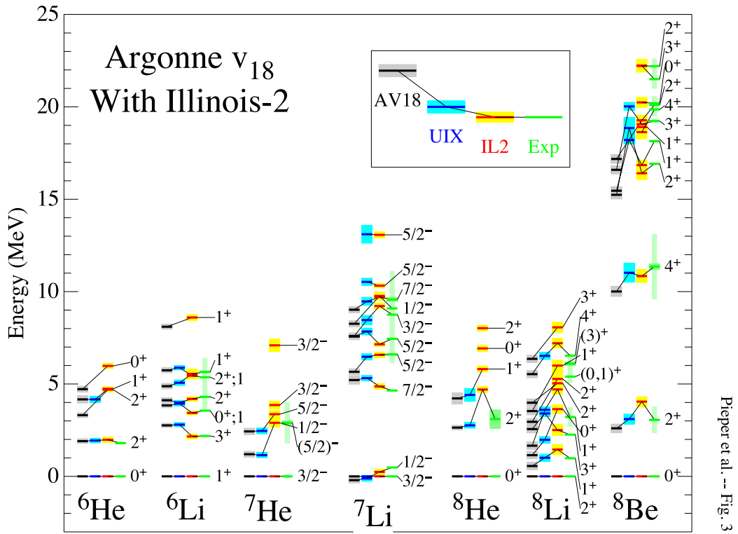
Figure 12: Green's Function Monte Carlo (GFMC) calculations for excited states in the A=6-8 region from [7]. This figure illustrates the precision achieved in these approaches. The energies of the ground states and lower excited states of the A=6-8 nuclei are plotted for several variants of Quantum Monte Carlo calculations, along with experimental data when it is available. The very small discrepancies between the IL2 approach and the excited states which have measured experimental values are typically less than 100 keV.
