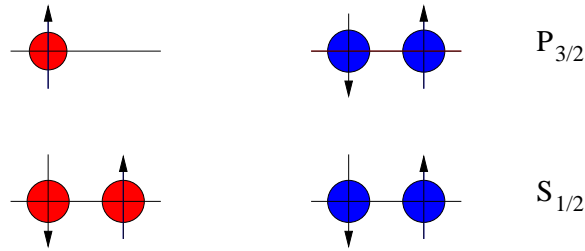
Figure 10: The shell model description of {}^7\text{Li} .
